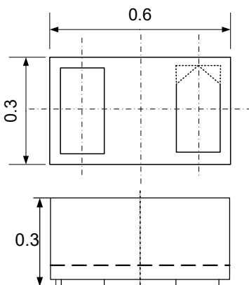
Package Dimensions
