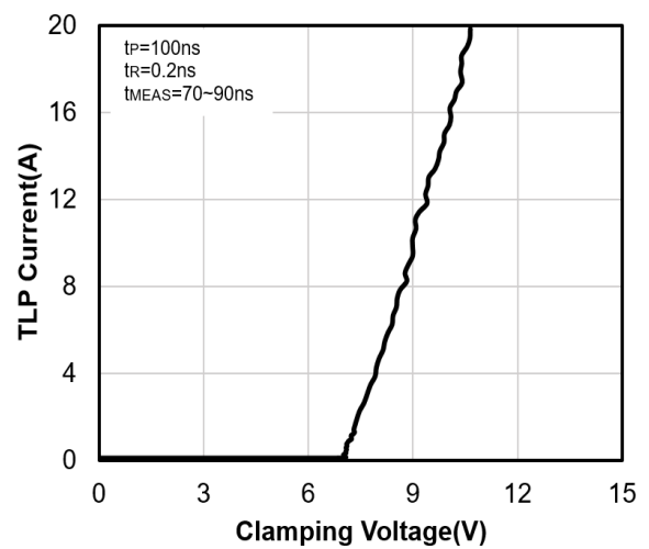
TLP Curve
